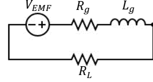
Fig. 2 Schematic of the knee energy harvester
