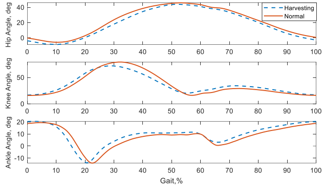
Fig. 9 Lower limb kinematics while walking at 6 km/h with and without the harvesting system
