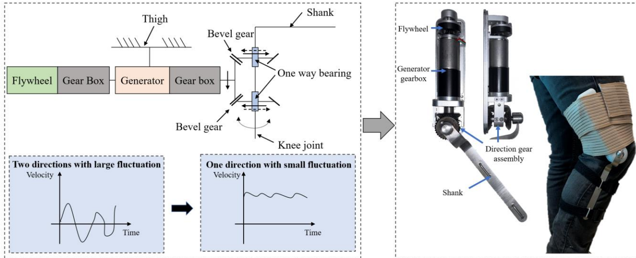
Fig. 1 (a) Schematic of the knee energy harvester and the desired outcome of the flywheel design (b) Harvester prototype layout and mounted on leg
