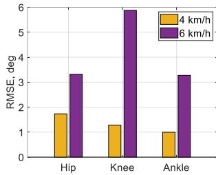
Fig. 10 Root mean square error between harvesting gait and normal gait
