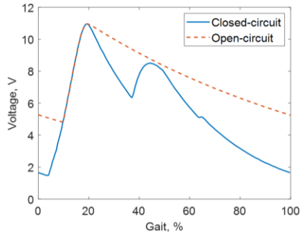
Fig. 3 Simulated harvester output voltage in open-circuit and closed-circuit mode with a 10\ \Omega load
