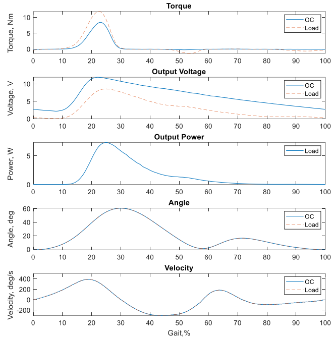
Fig. 5 Output of the harvesting system over a gait
