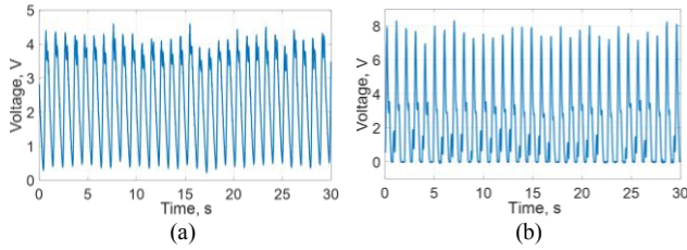
Fig. 7 Open-circuit voltage after rectification when walking at 6 km/h with (a) flywheel and (b) conventional harvester
