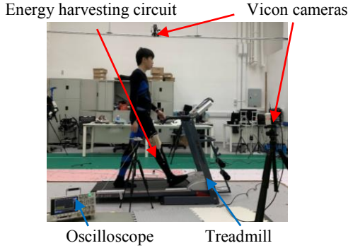
Fig. 6 Experimental setup for harvester evaluation
