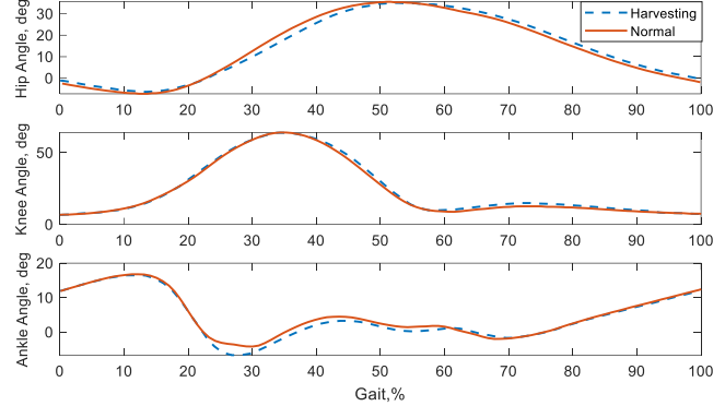
Fig. 8 Lower limb kinematics while walking at 4 km/h with and without the harvesting system
