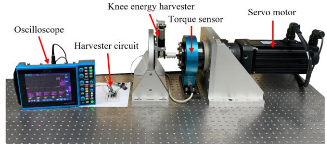
Fig. 4 Setup of the harvester testbench
